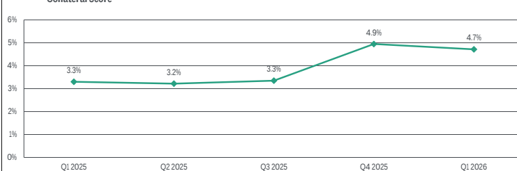
Chart 6: Collateral Score
